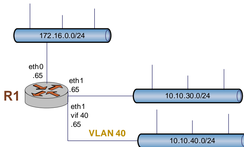
Figure 1-3 VLAN configuration
